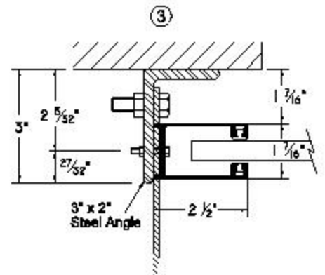
Minimum Clearance From Face of Guide
